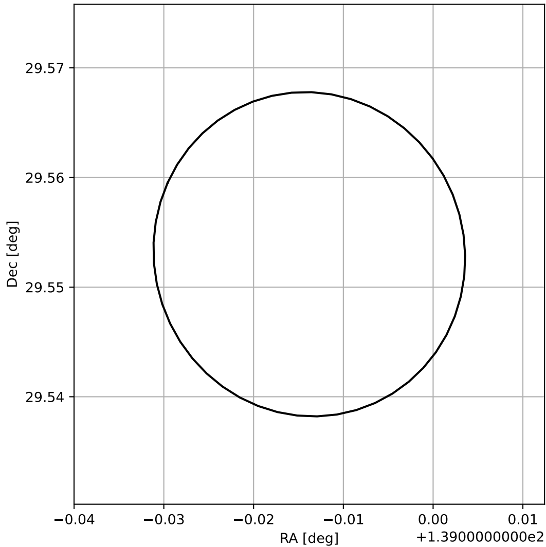
4FGL J0915.9+2933
