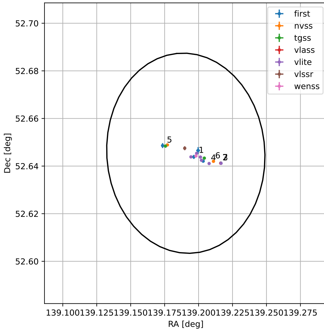
4FGL J0916.7+5238
