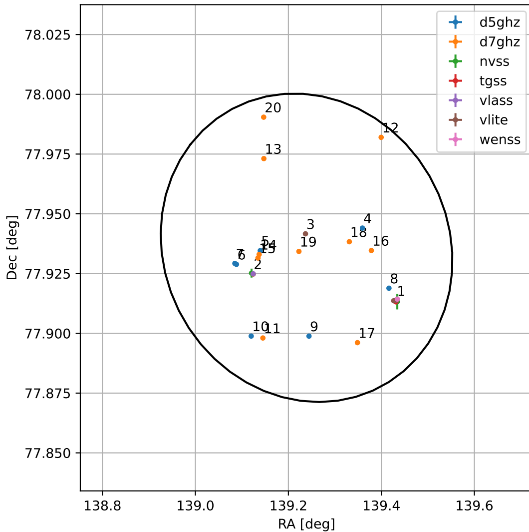
4FGL J0916.9+7756
