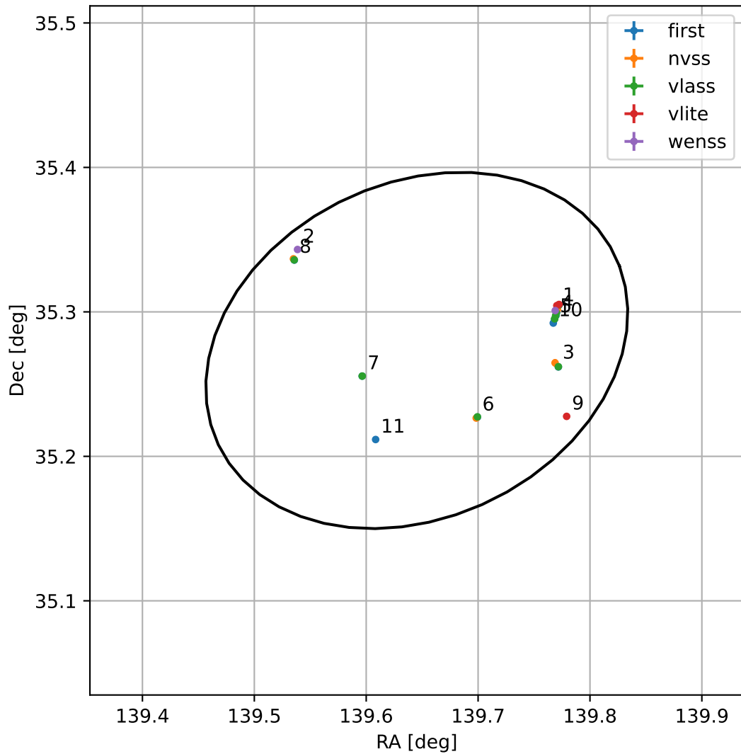
4FGL J0918.5+3516
