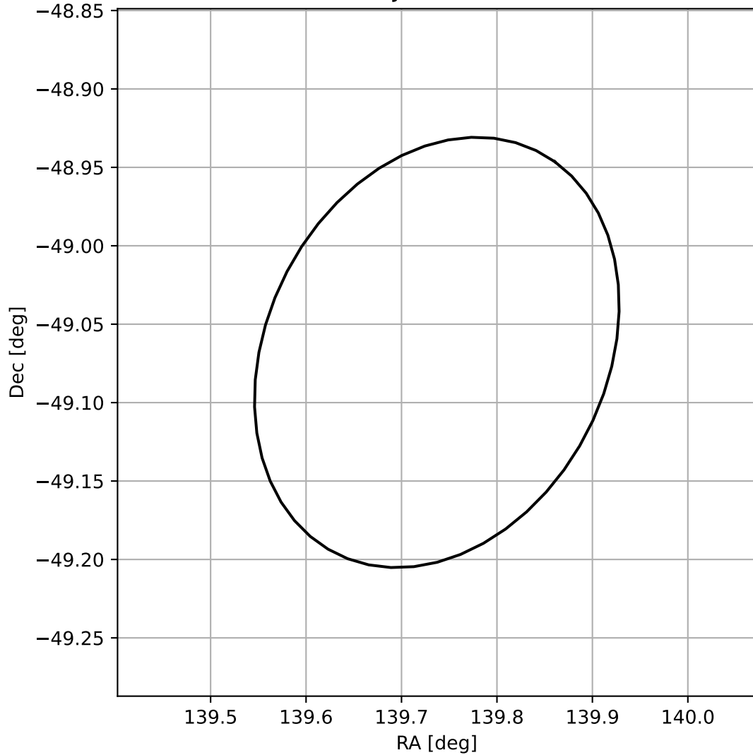
4FGL J0918.9-4904
