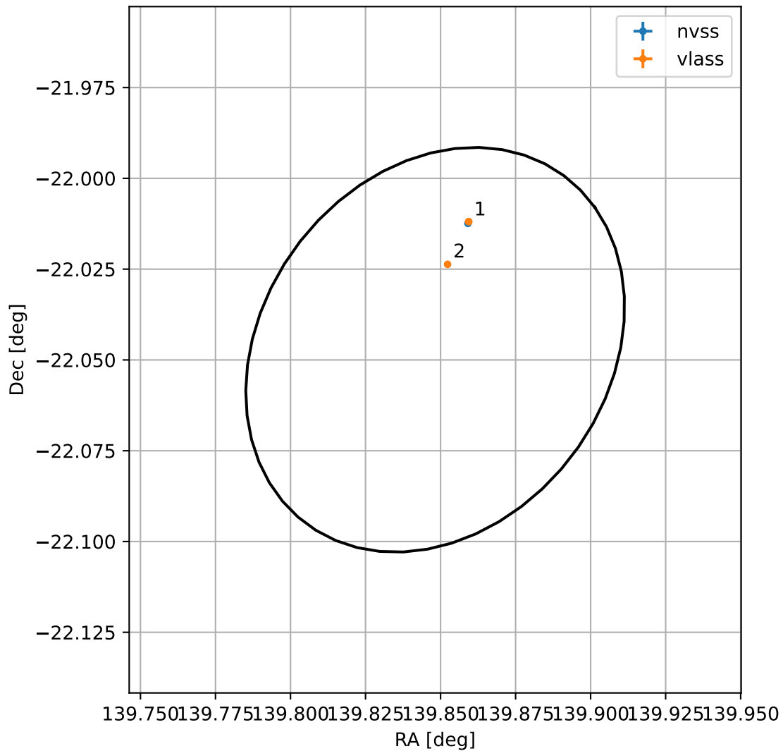
4FGL J0919.3-2202
