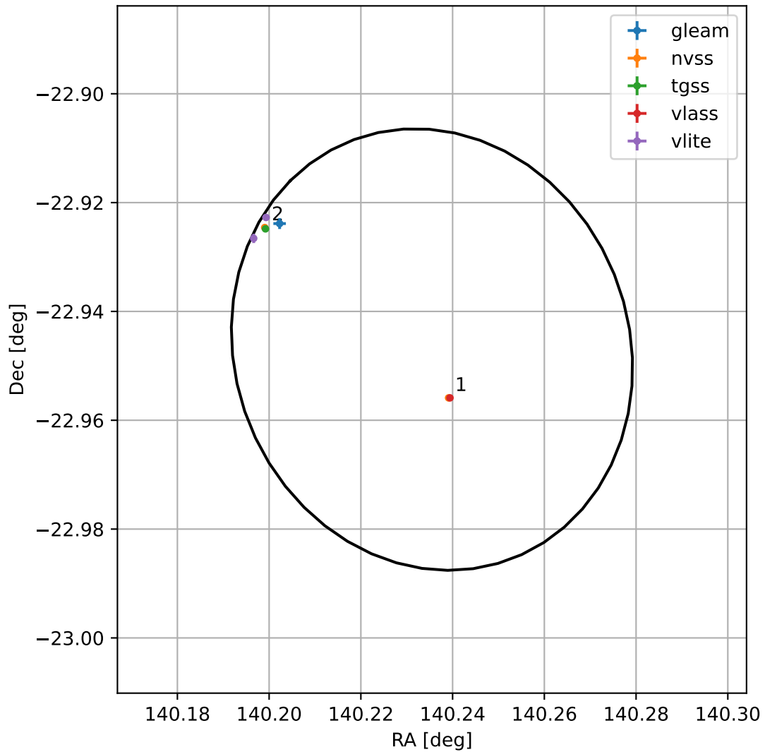
4FGL J0920.9-2256
