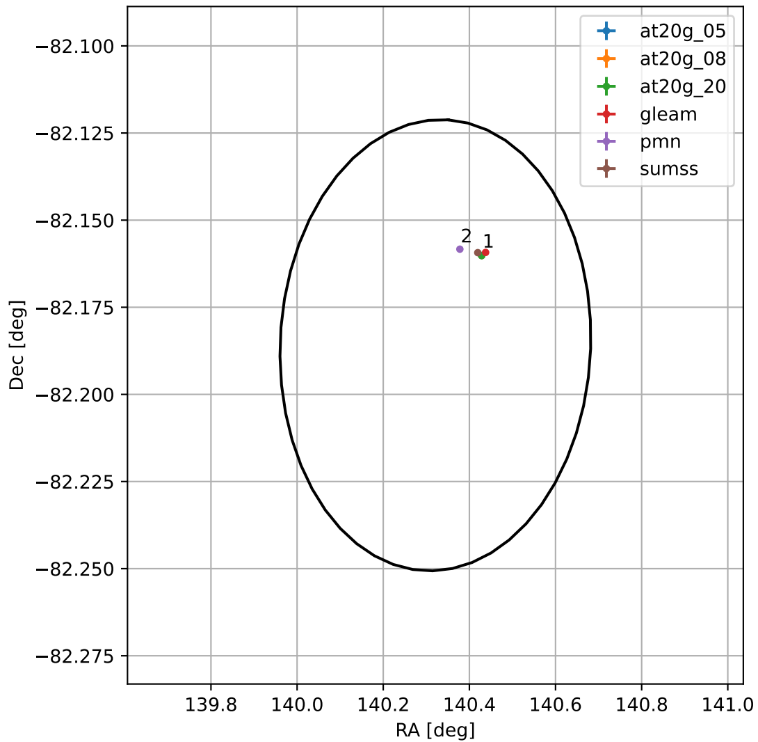
4FGL J0921.2-8211
