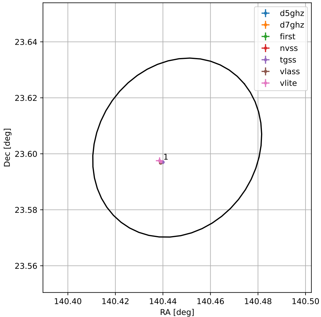
4FGL J0921.7+2336
