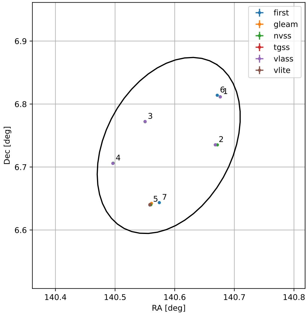
4FGL J0922.3+0644
