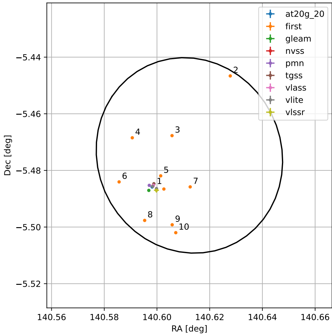
4FGL J0922.4-0528
