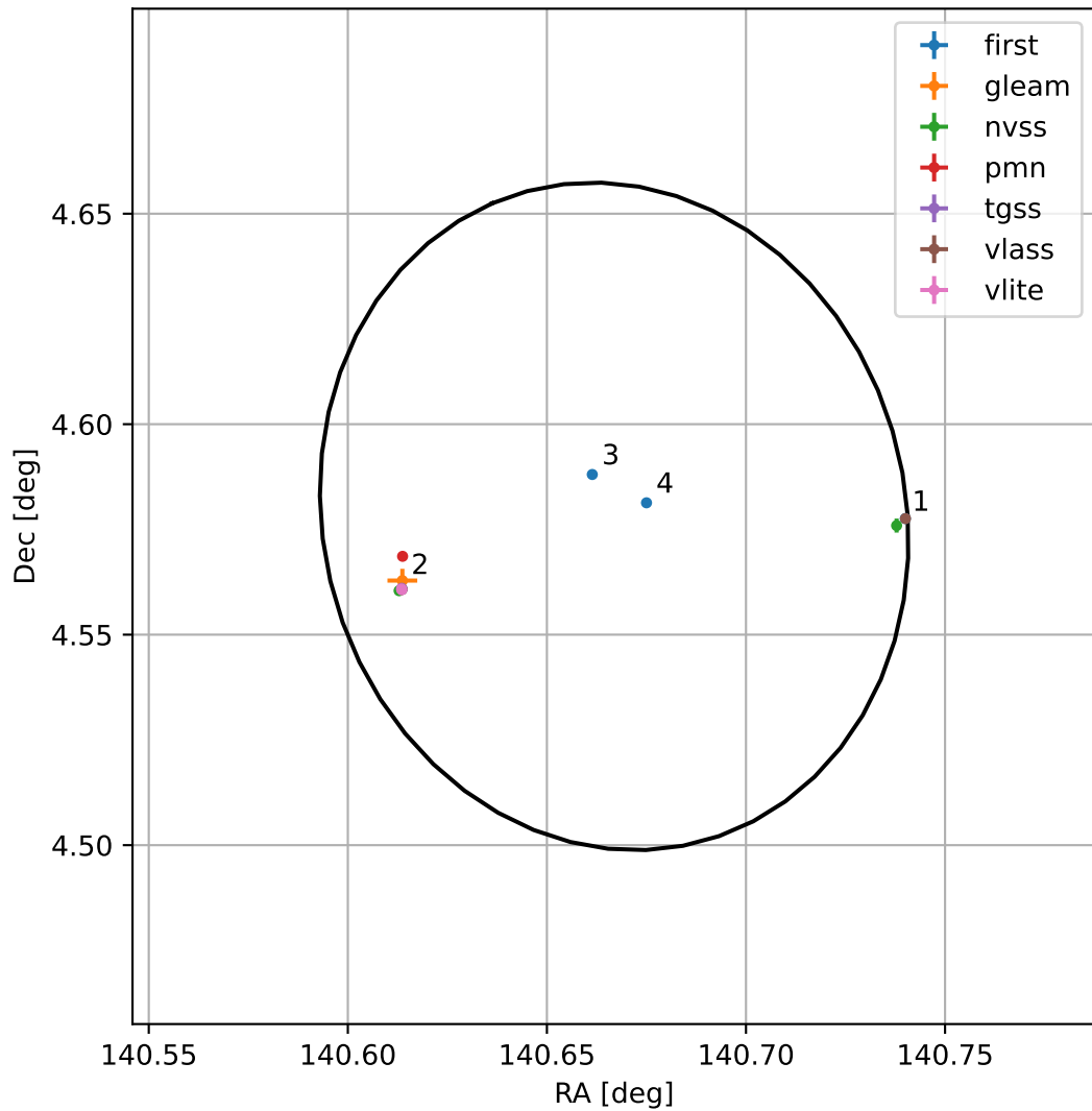
4FGL J0922.6+0434
