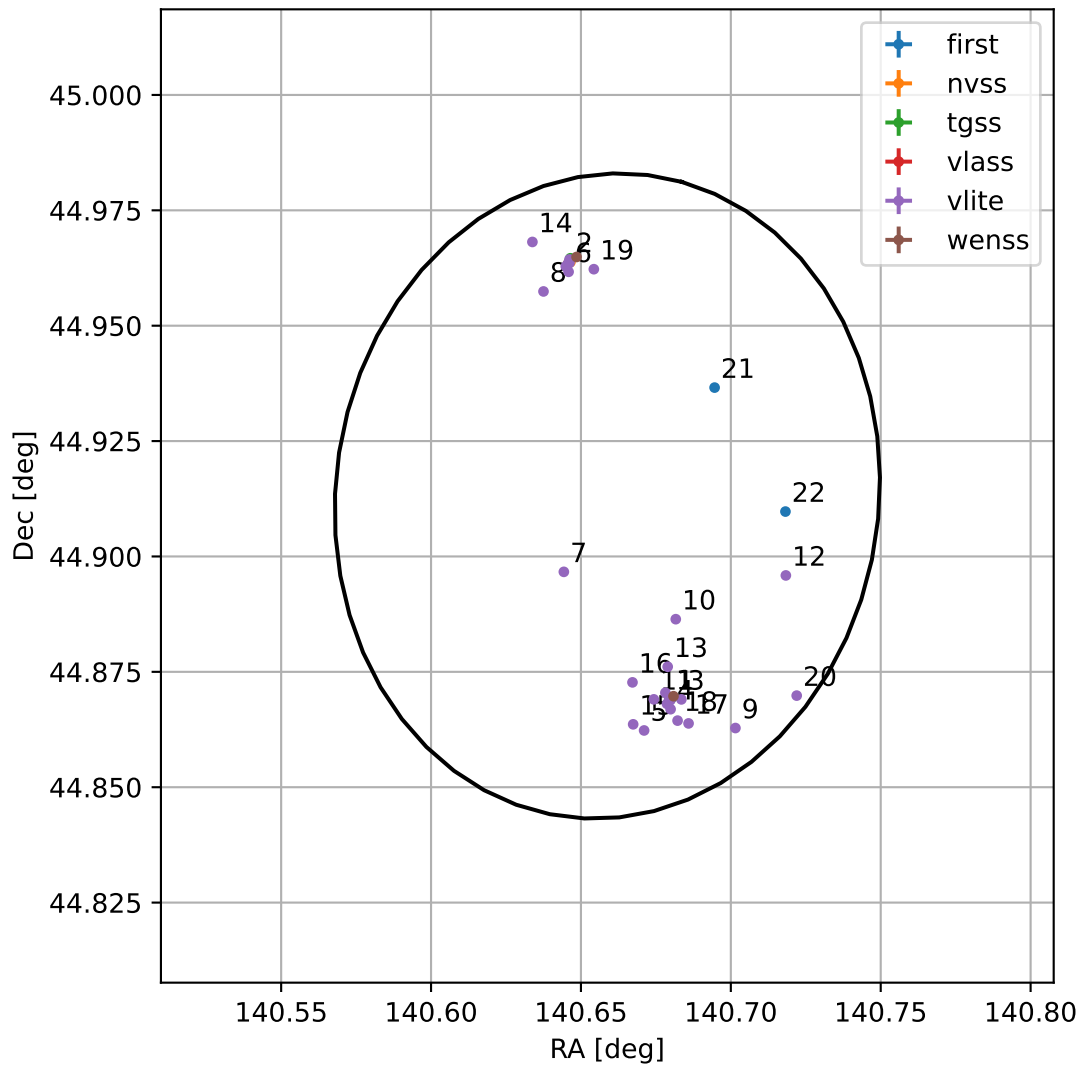
4FGL J0922.6+4454
