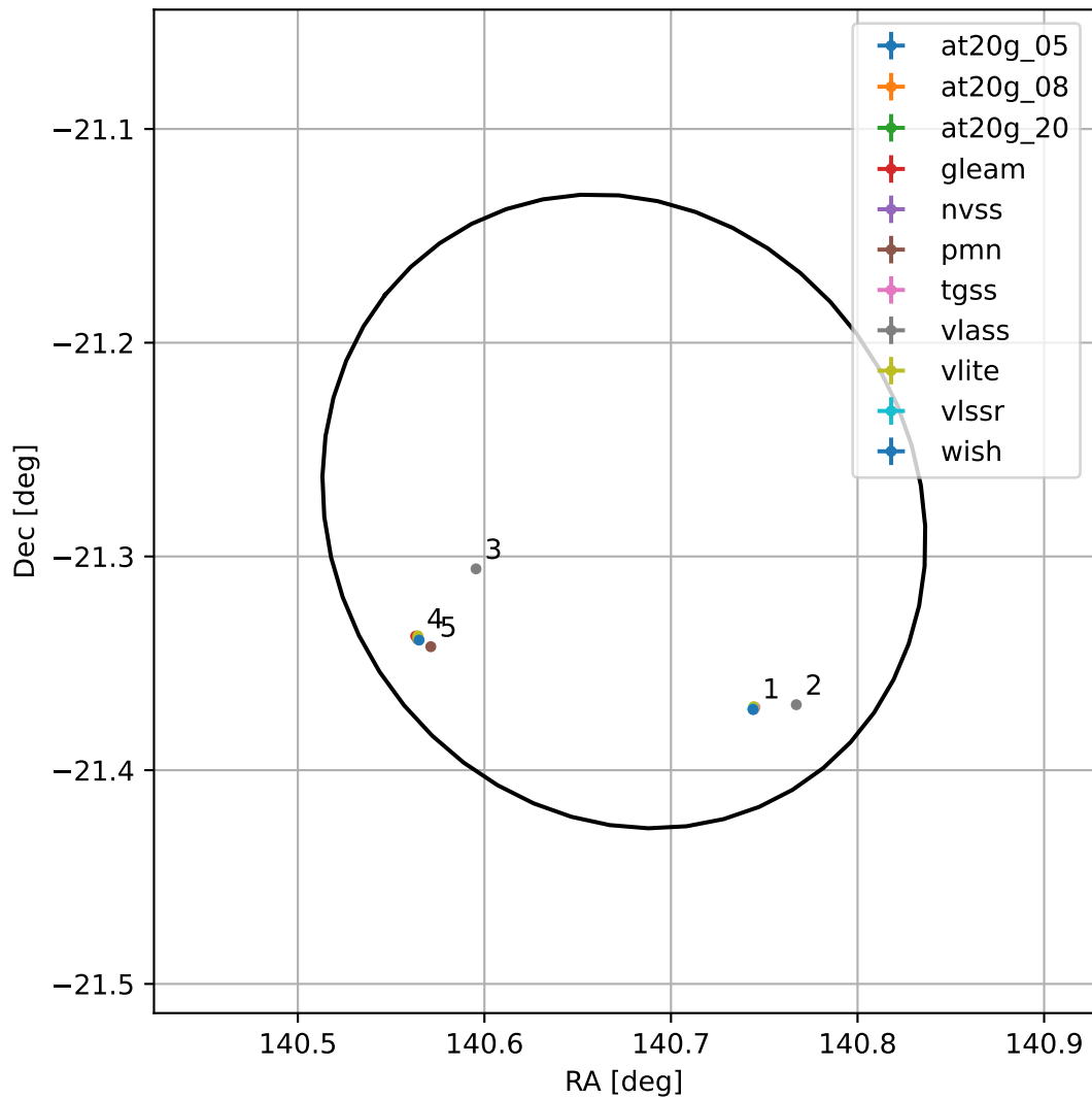
4FGL J0922.6-2116
