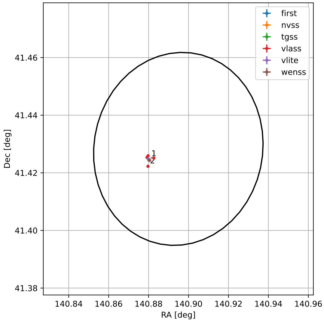
4FGL J0923.5+4125
