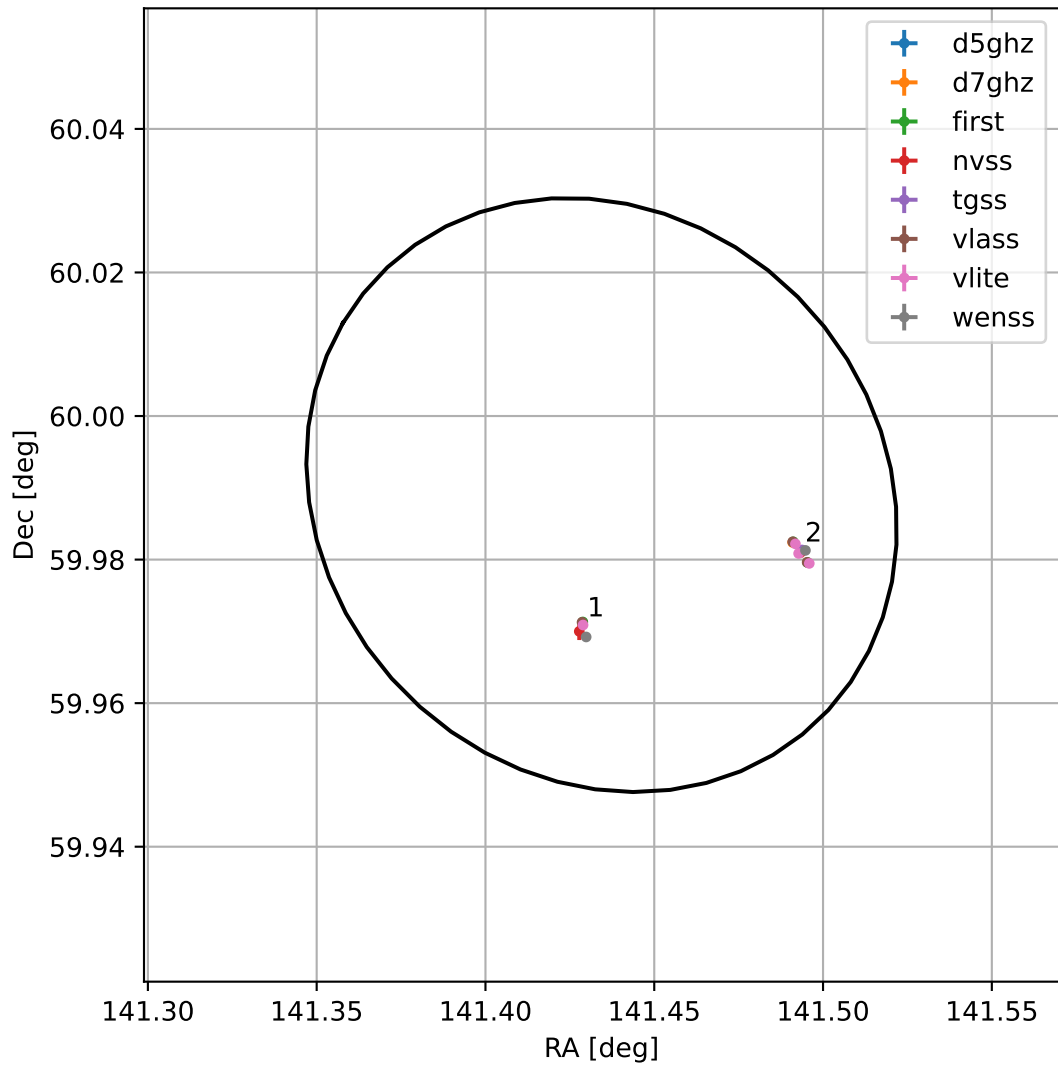
4FGL J0925.7+5959
