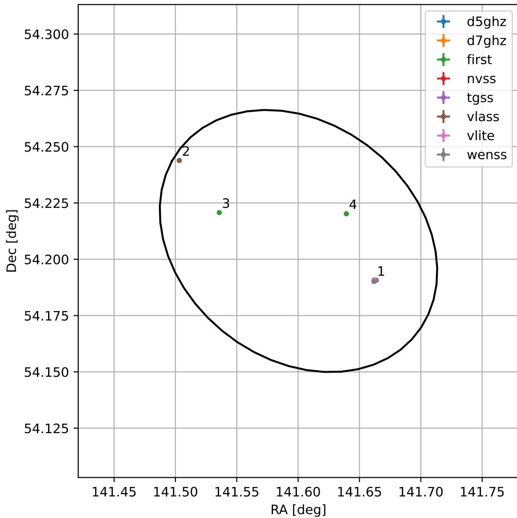
4FGL J0926.4+5412
