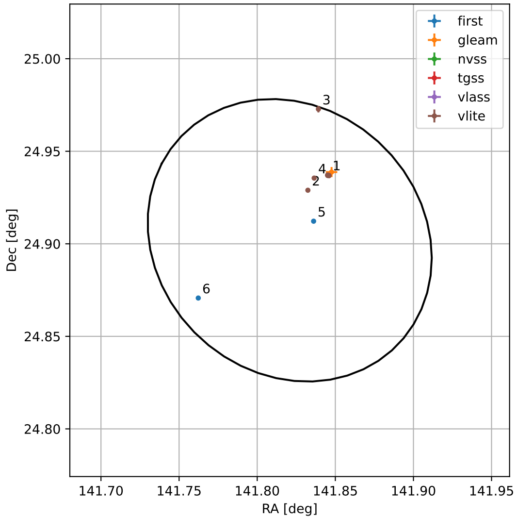
4FGL J0927.2+2454
