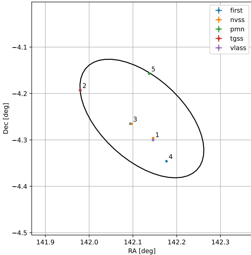
4FGL J0928.4-0415
