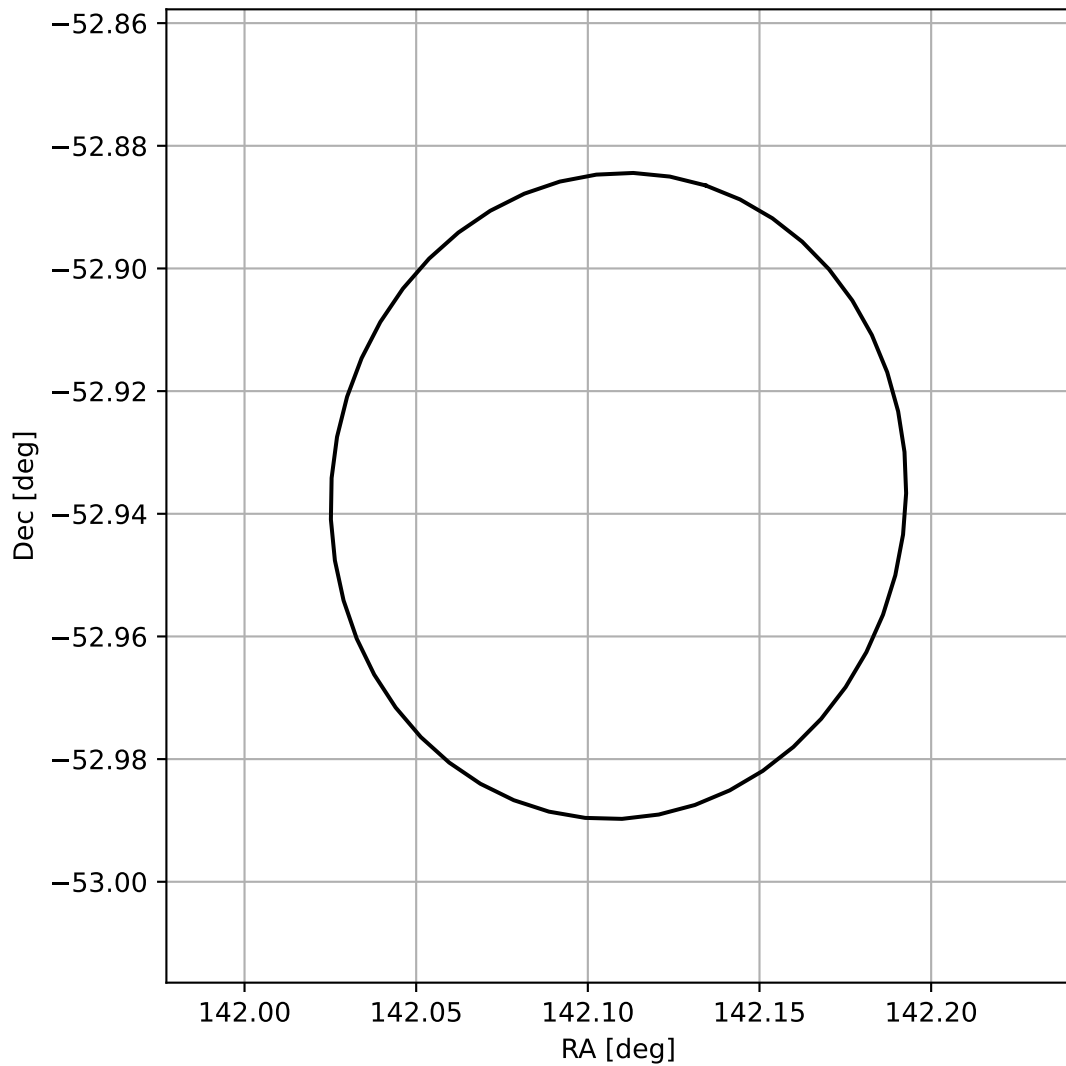
4FGL J0928.4-5256
