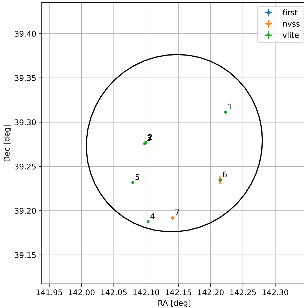
4FGL J0928.5+3916
