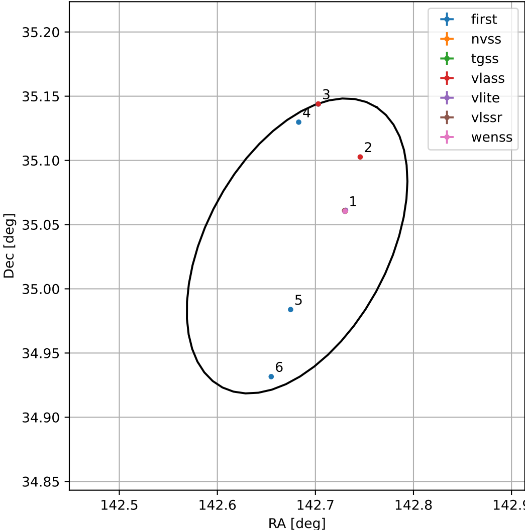
4FGL J0930.7+3502
