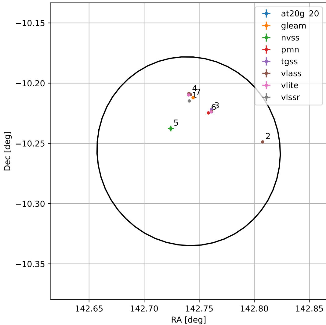
4FGL J0930.9-1015
