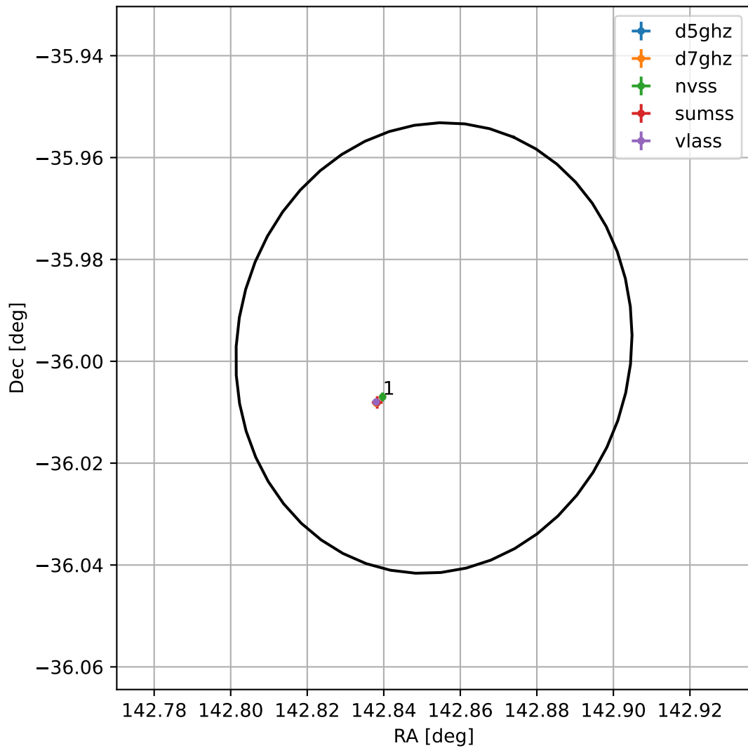
4FGL J0931.4-3559
