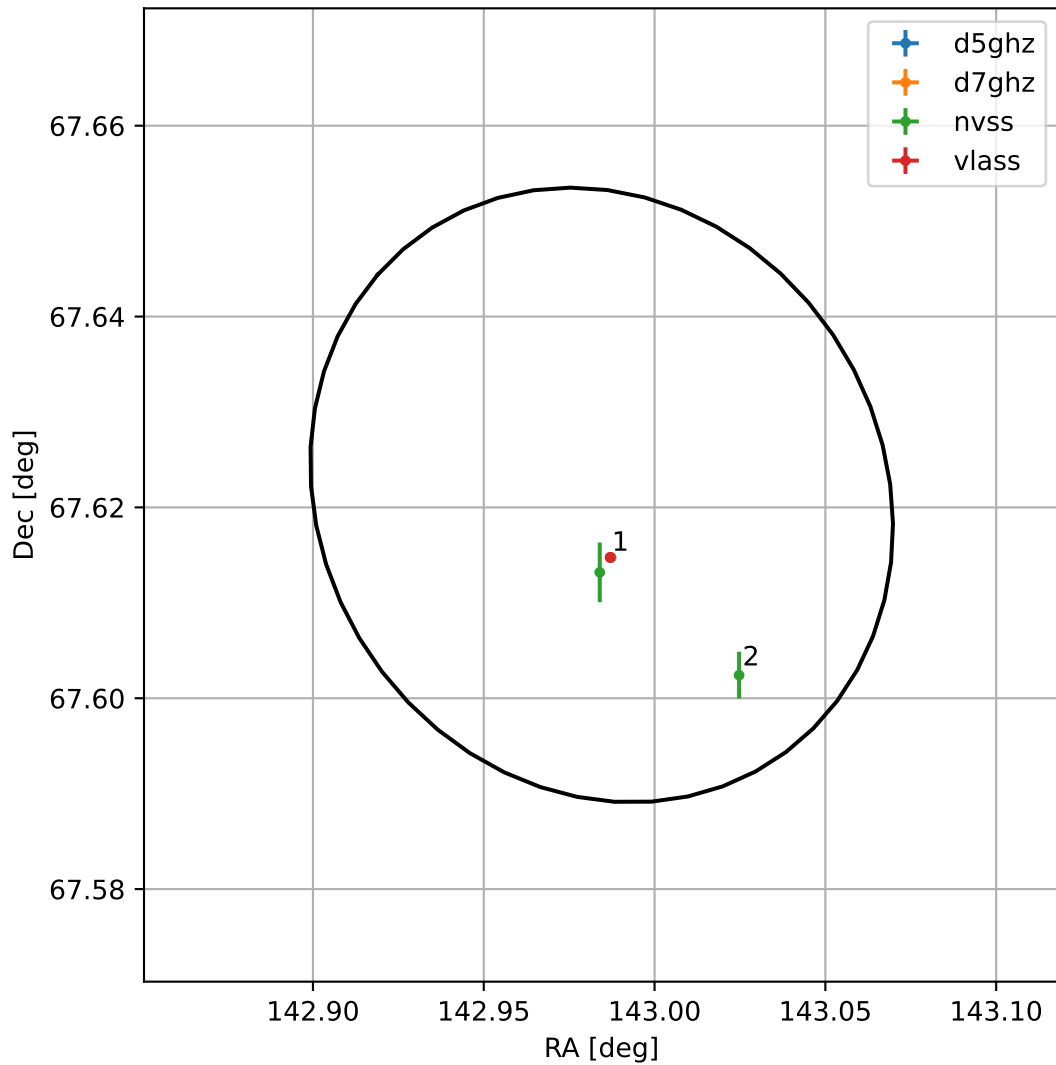
4FGL J0931.9+6737
