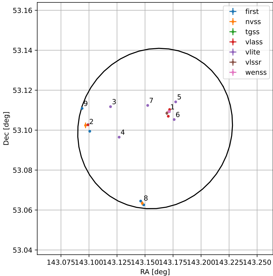
4FGL J0932.6+5306
