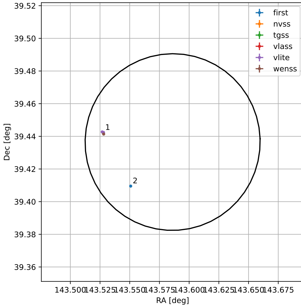
4FGL J0934.3+3926
