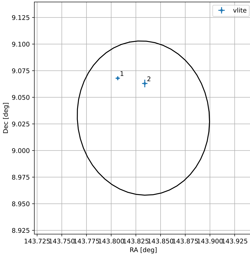
4FGL J0935.3+0901
