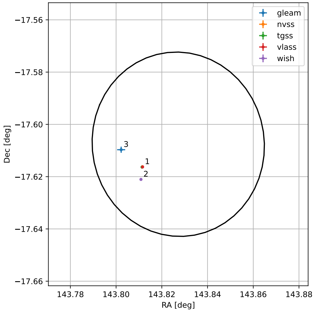
4FGL J0935.3-1736
