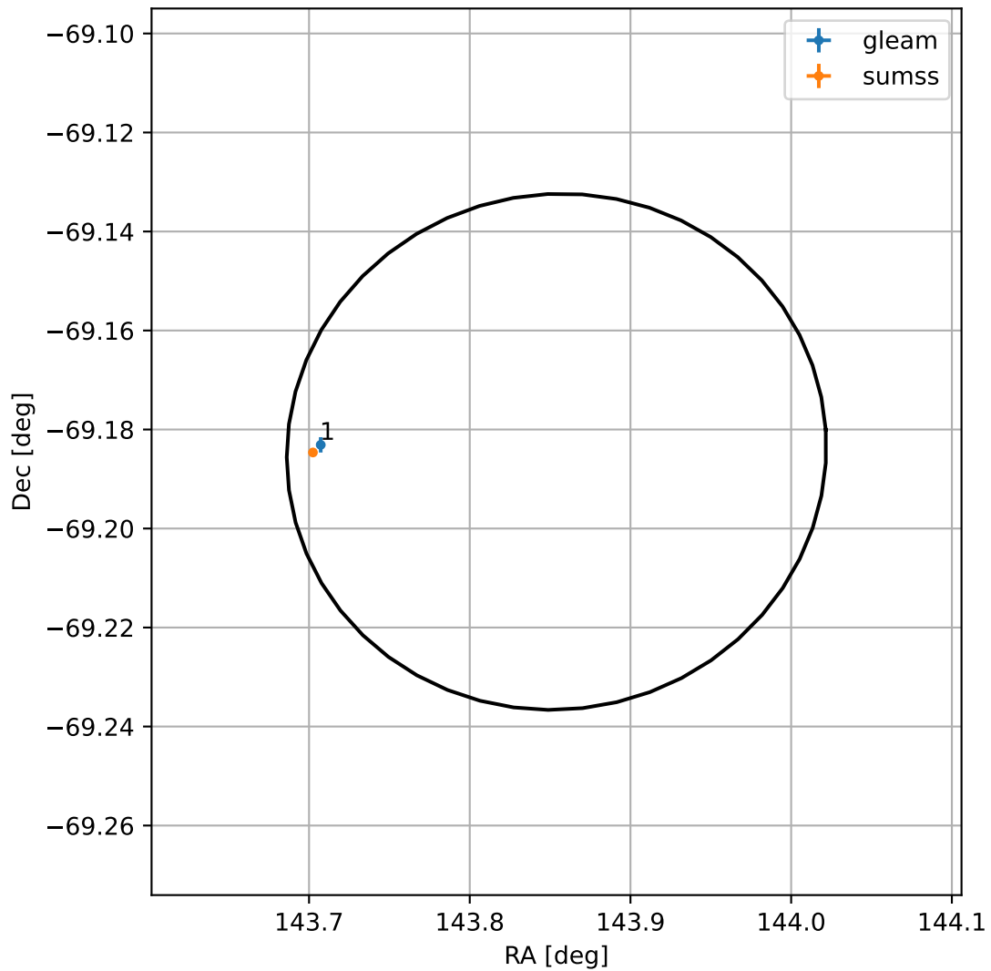
4FGL J0935.4-6911
