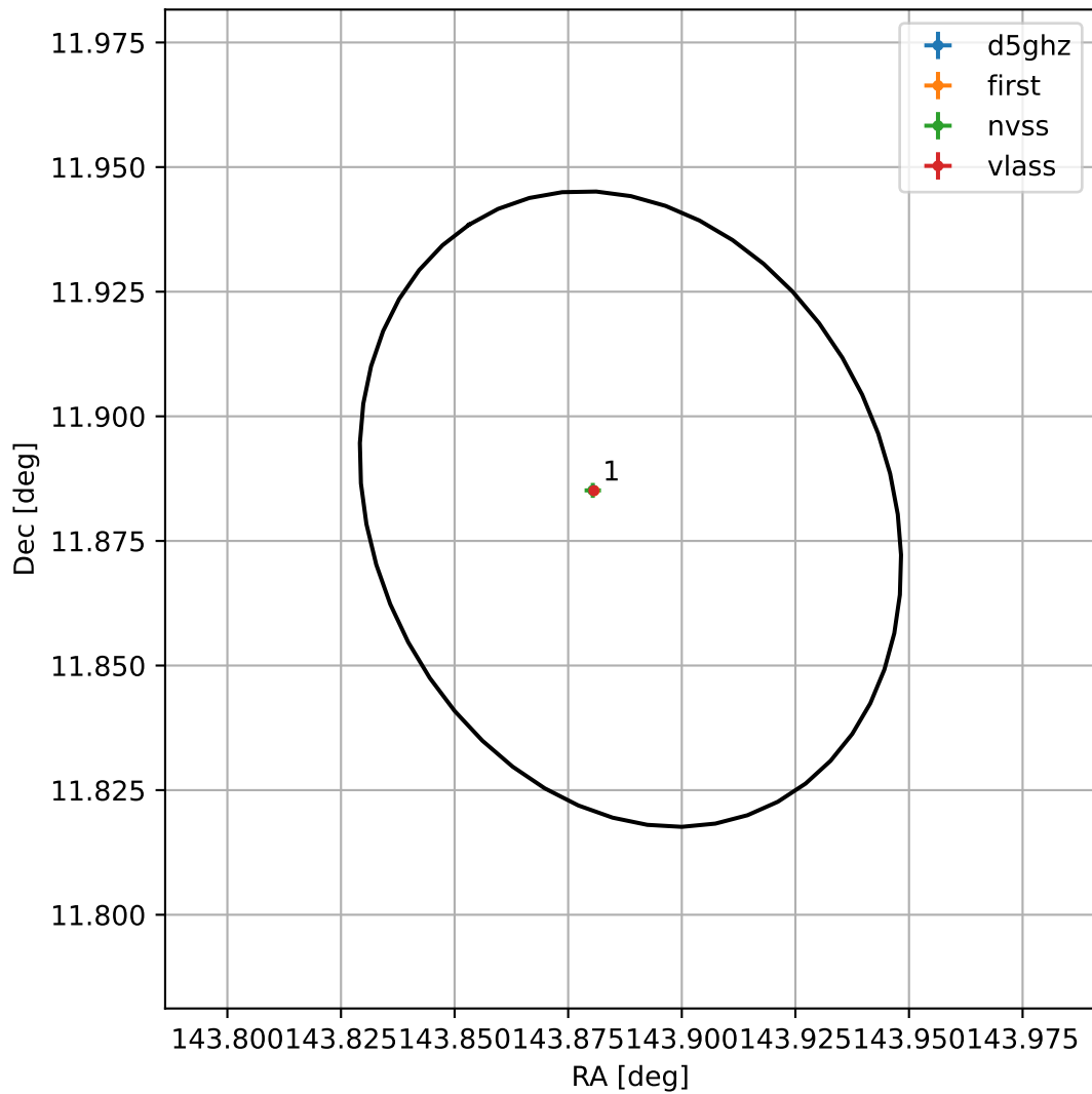
4FGL J0935.5+1152
