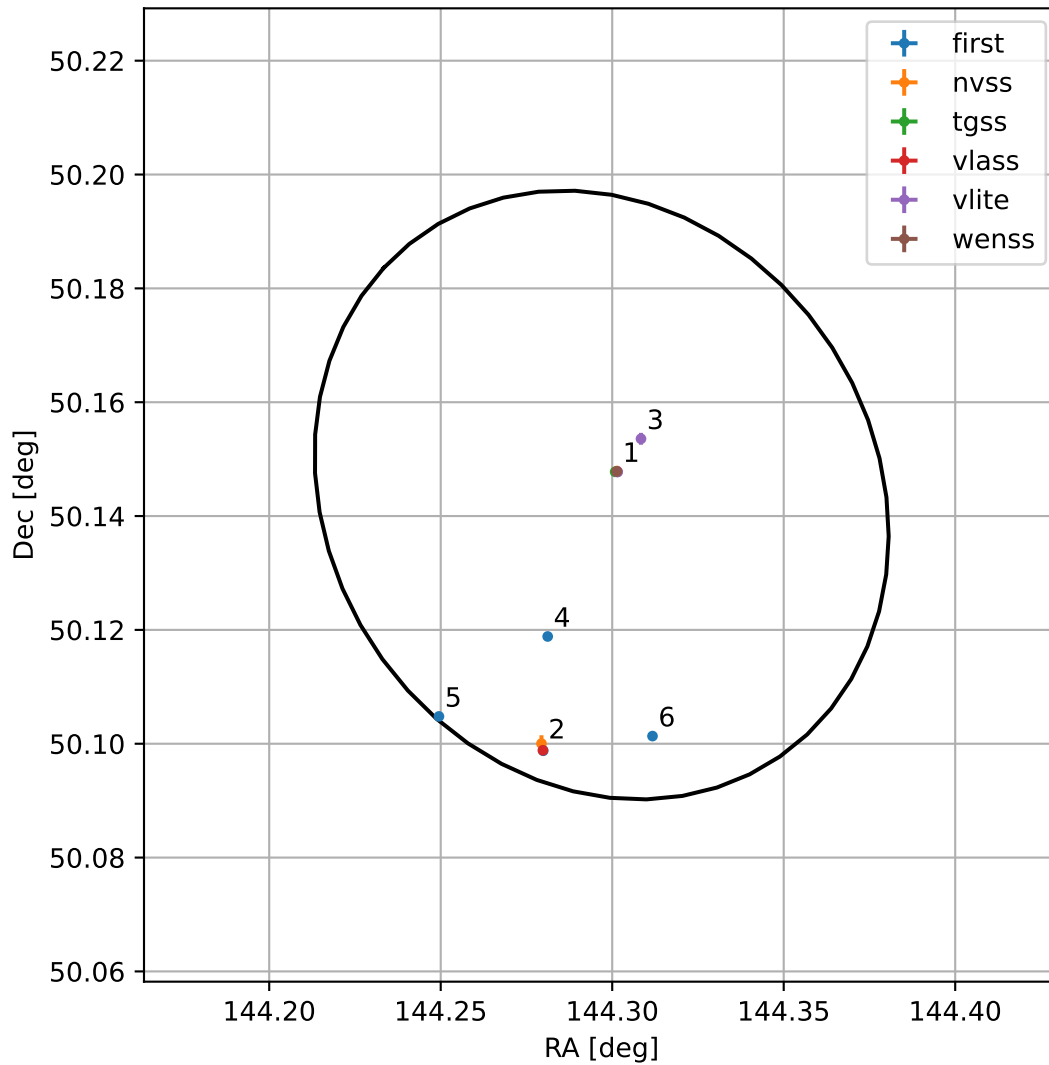
4FGL J0937.1+5008
