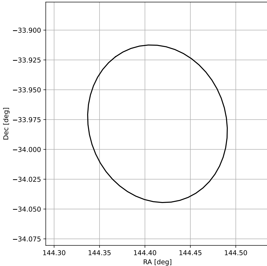
4FGL J0937.6-3358
