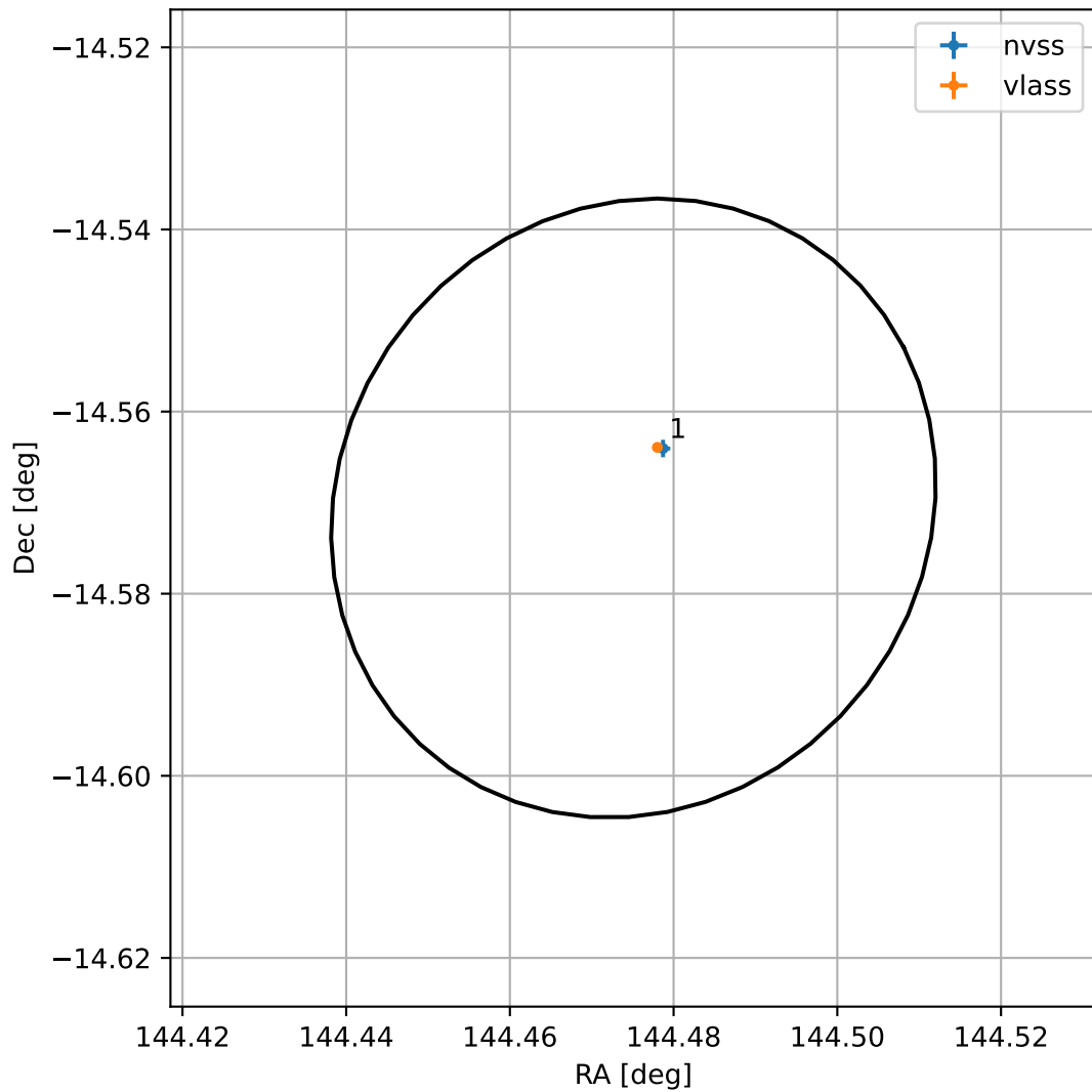
4FGL J0937.9-1434
