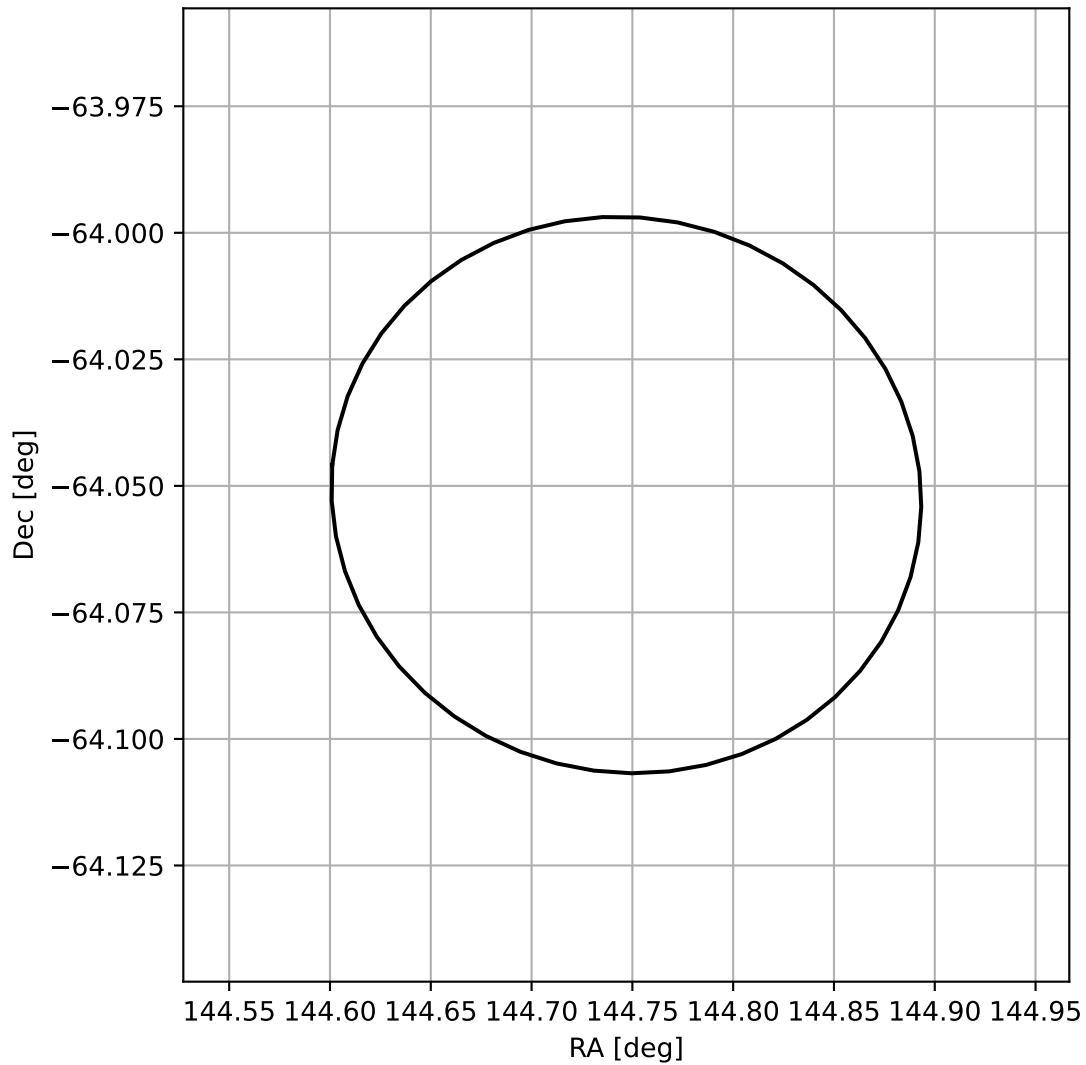
4FGL J0938.9-6403
