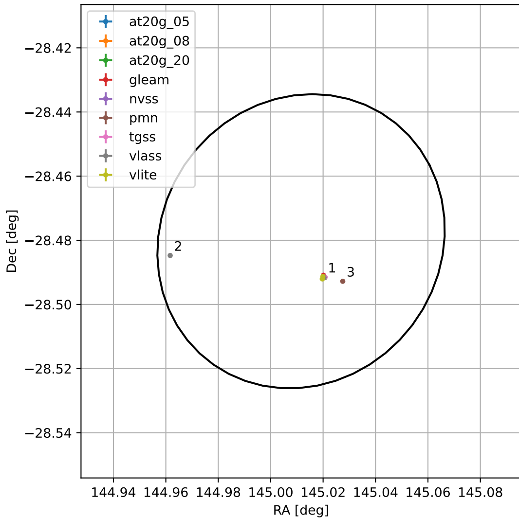
4FGL J0940.0-2828
