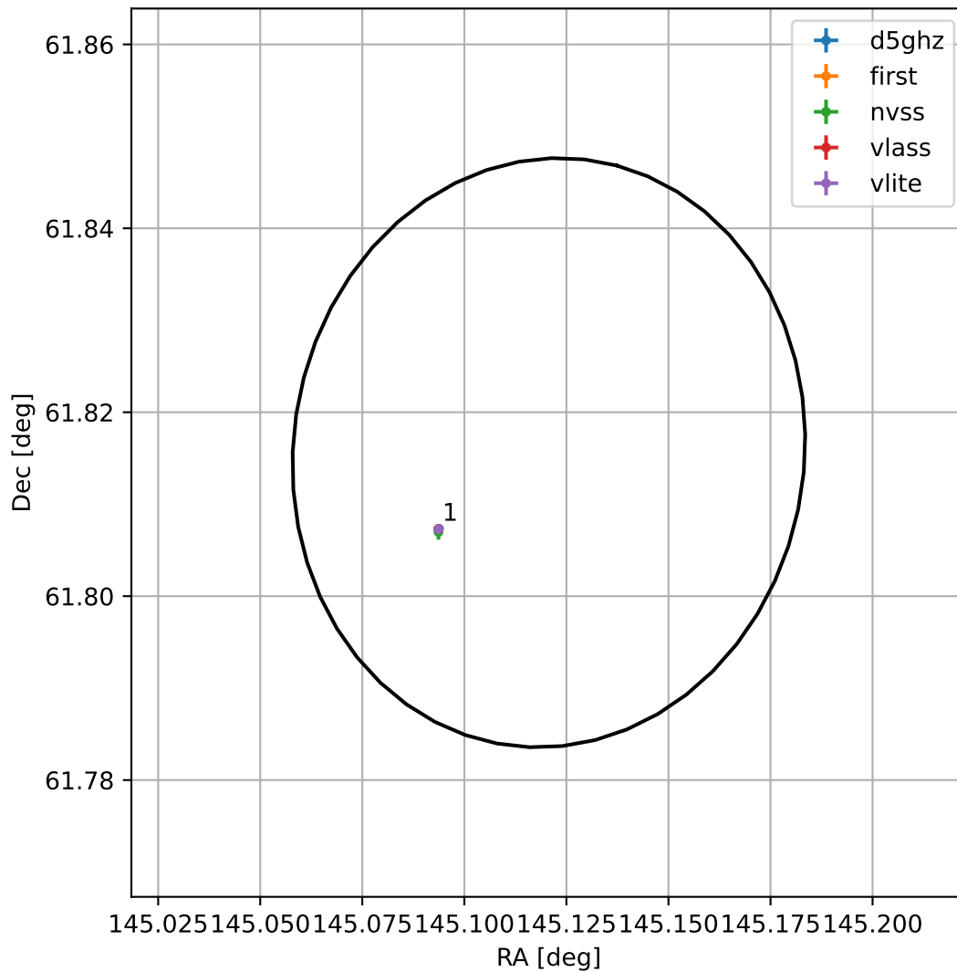
4FGL J0940.4+6148
