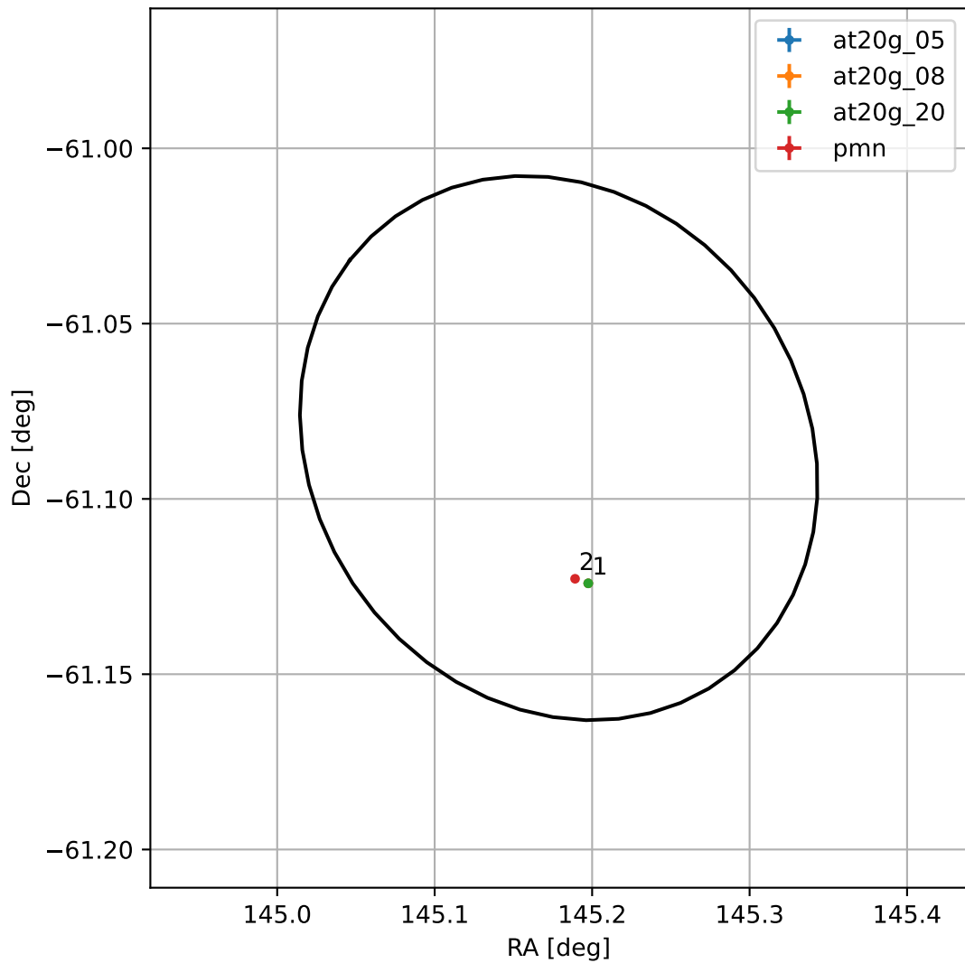
4FGL J0940.7-6105
