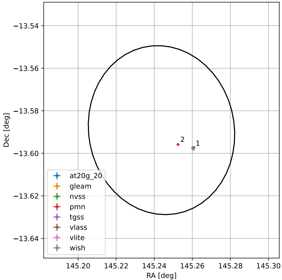
4FGL J0940.9-1335
