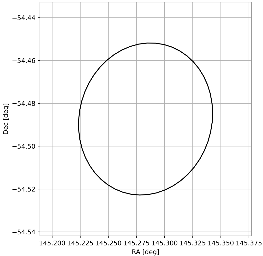
4FGL J0941.1-5429
