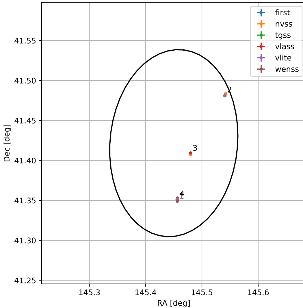
4FGL J0941.7+4125
