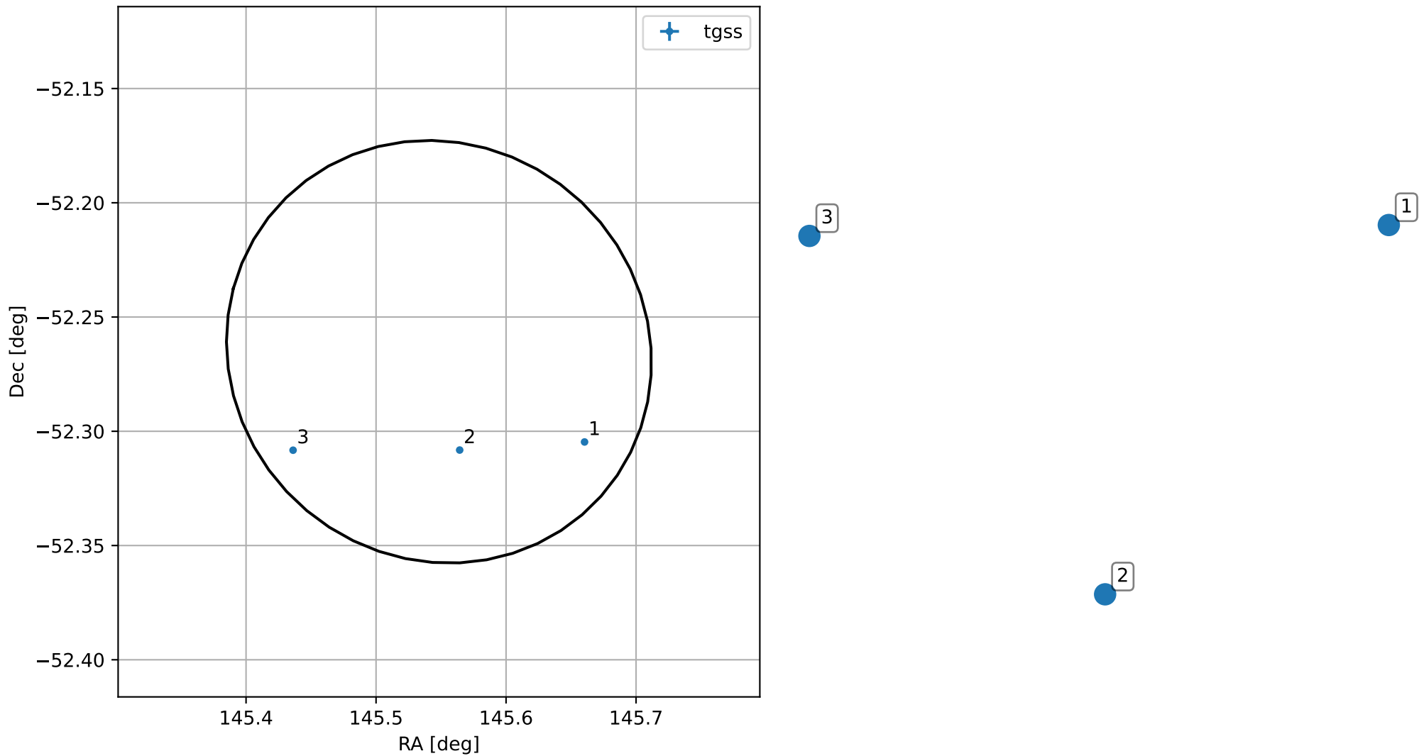
4FGL J0942.1-5215
