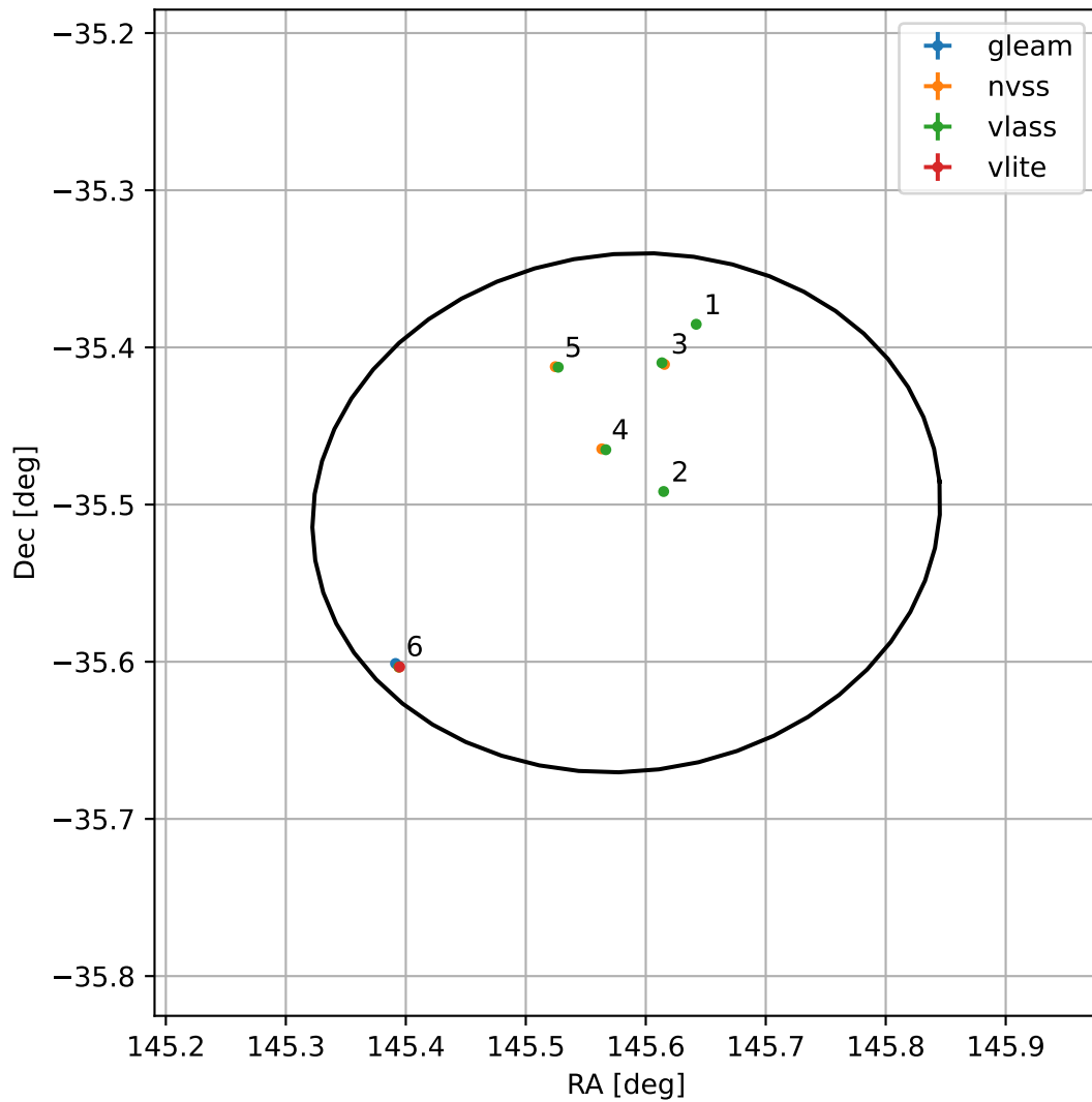
4FGL J0942.3-3530
