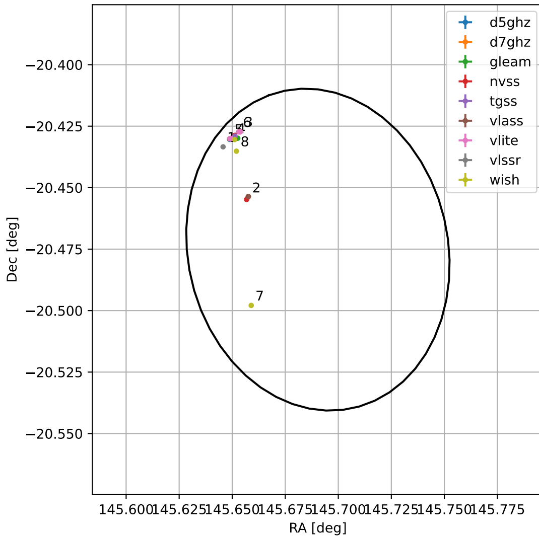
4FGL J0942.7-2028
