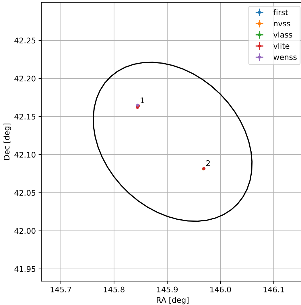
4FGL J0943.6+4207
