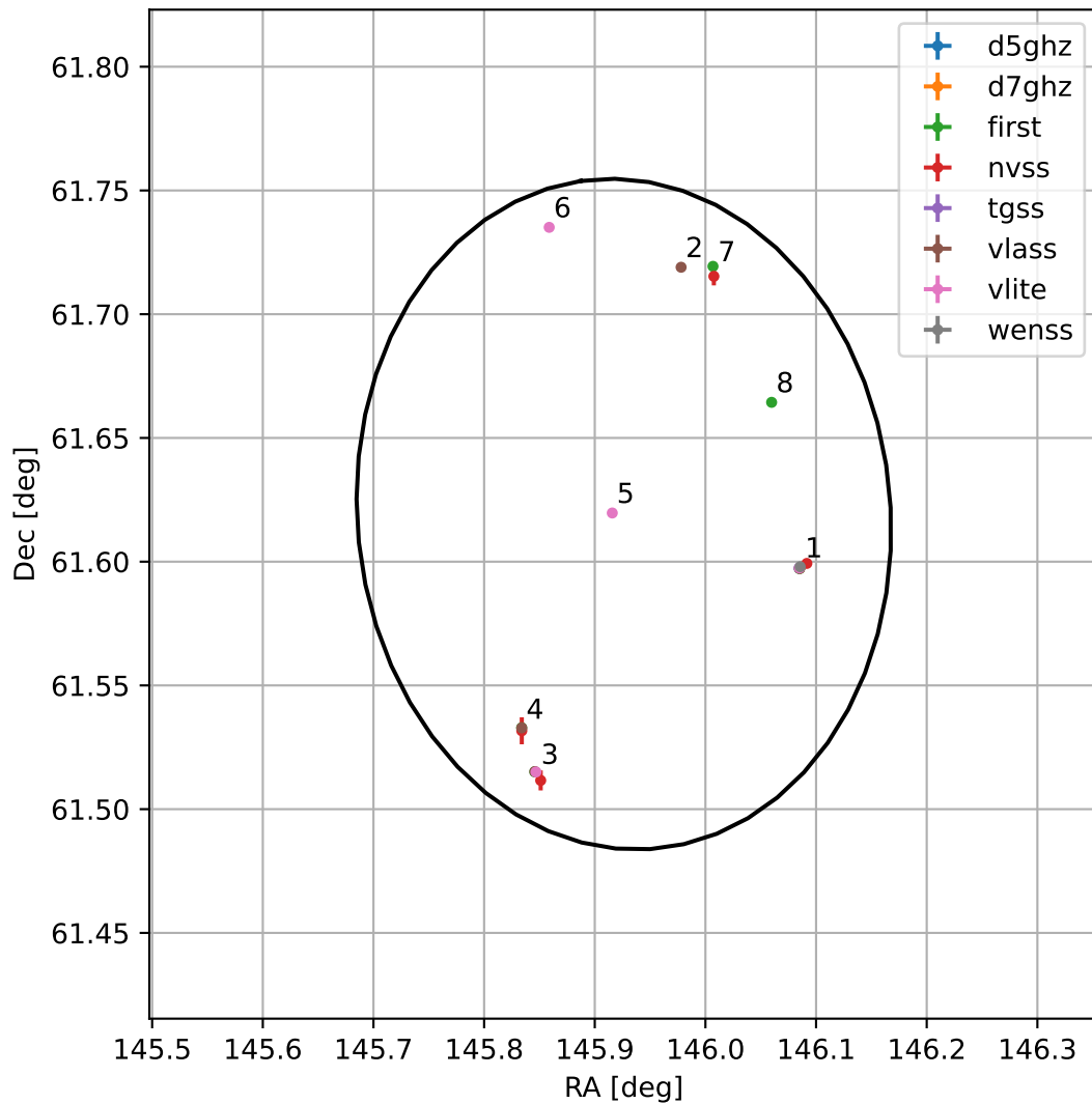
4FGL J0943.7+6137
