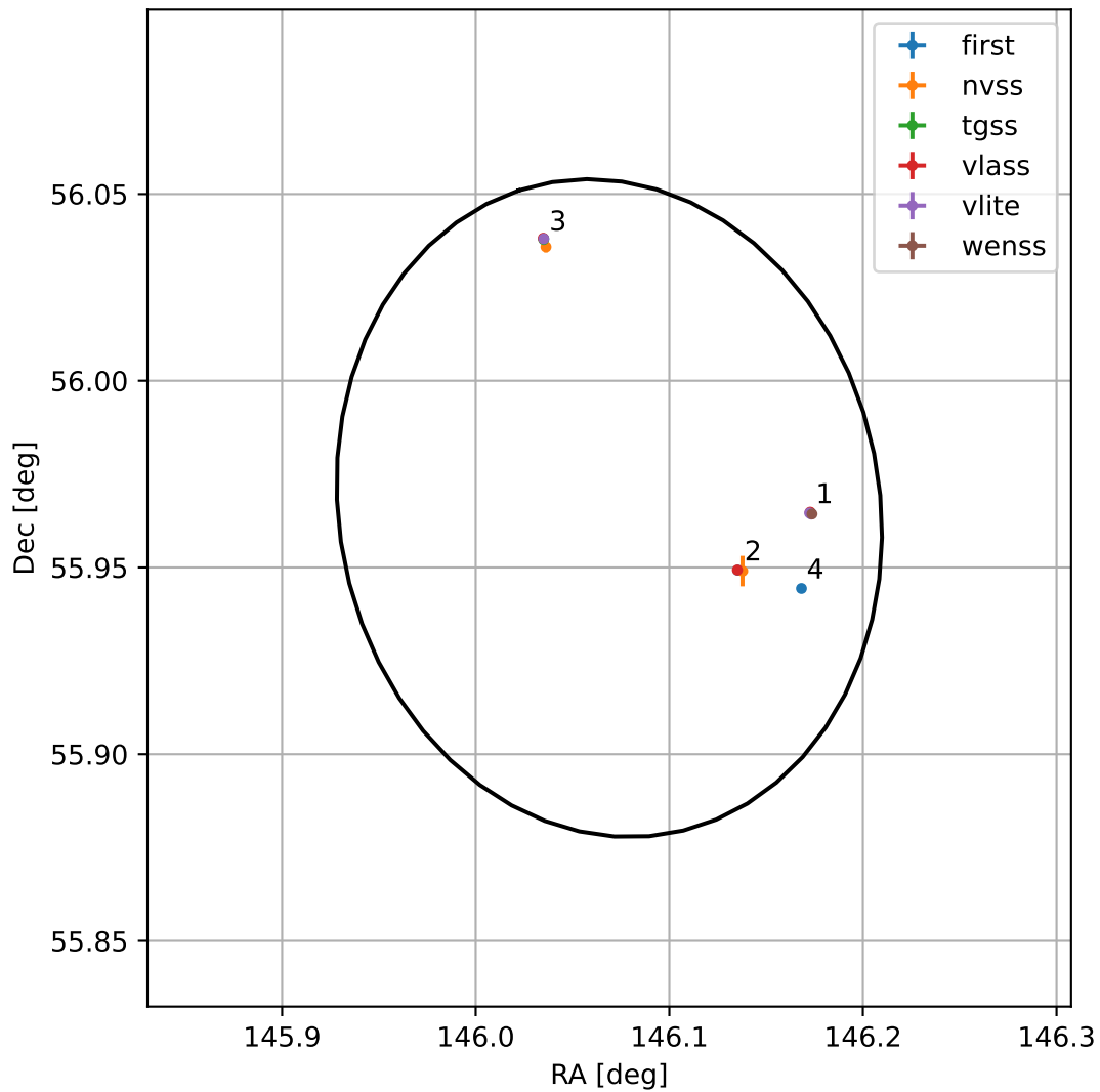
4FGL J0944.2+5557
