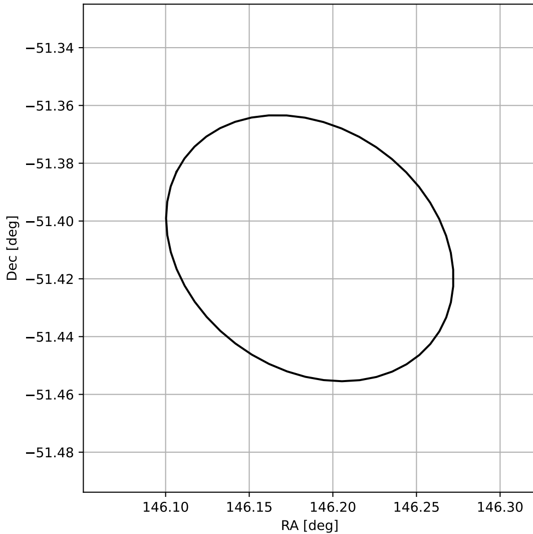
4FGL J0944.7-5124
