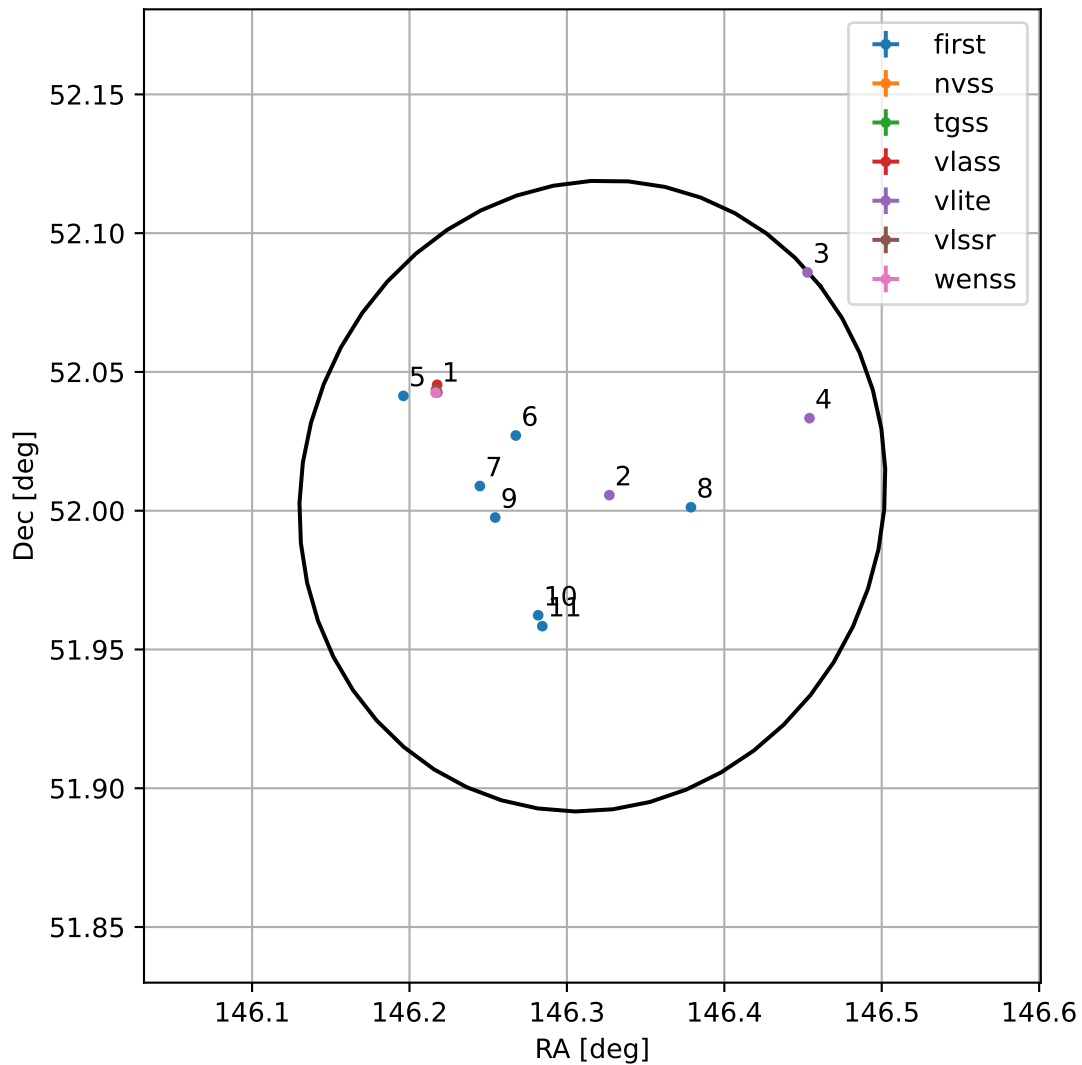
4FGL J0945.2+5200
