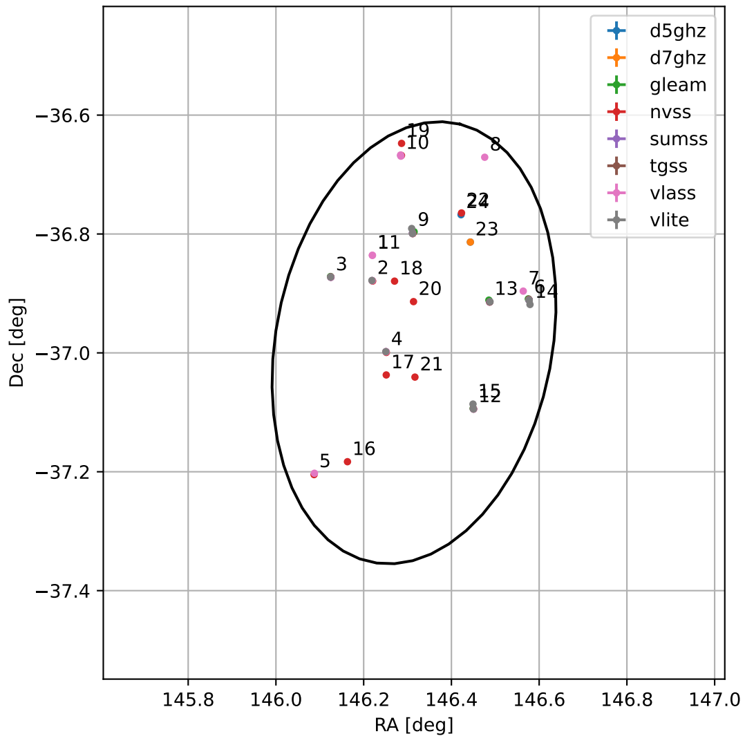
4FGL J0945.2-3658
